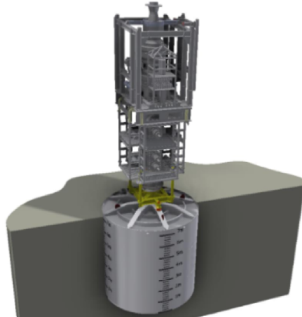
Suction Anchor
